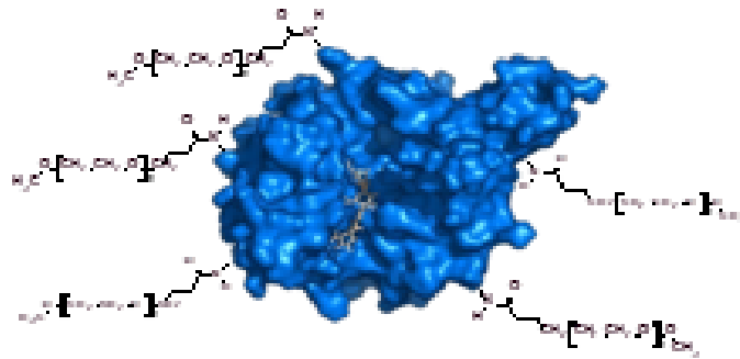
PEGylated form of rHuPH20
